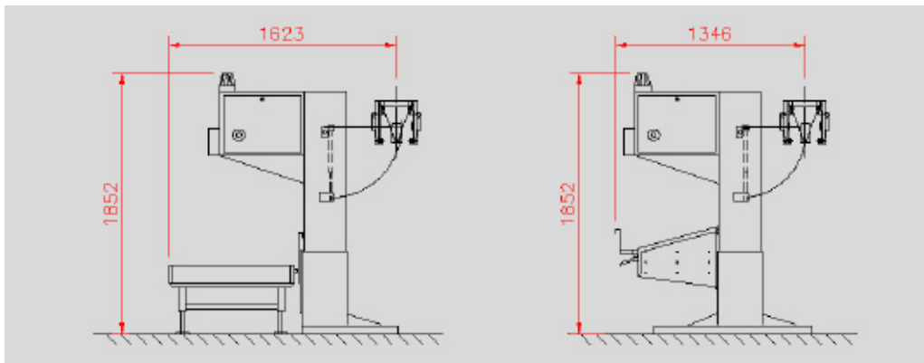
Typical Dimensions Shown, Equipment Manufactured To Suit Each Installation.
