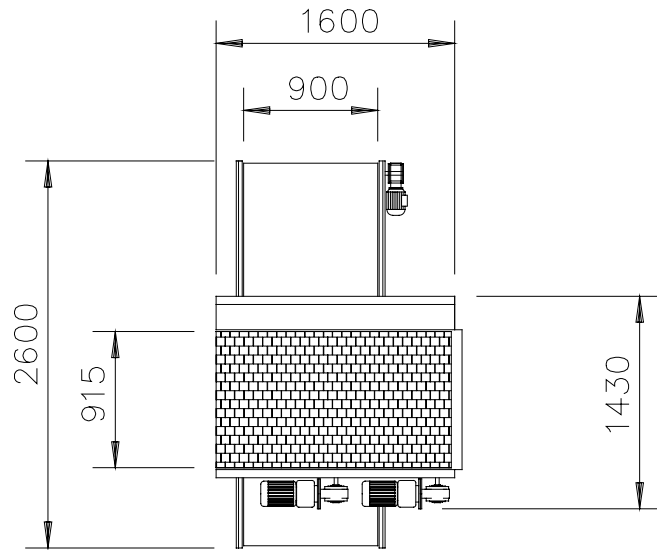
Screen Grading Module, available from 600mm wide to 2400mm wide
