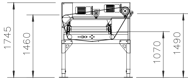
Screen Grading Module, available from 600mm wide to 2400mm wide
